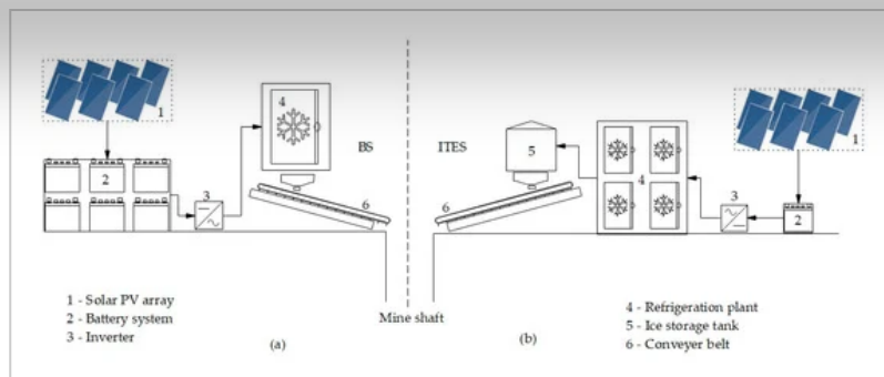
Figure 1. (a). Flow schematics of Battery Storage System (BS) and (b). Flow schematic of Ice Thermal Energy Storage System (ITES).
