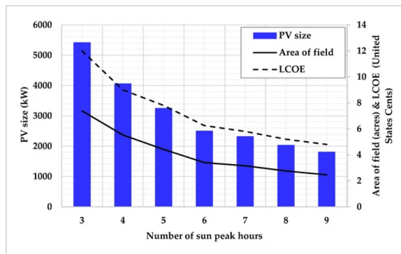
Figure 2. PV size, Levelized Cost of Energy (LCOE), and area variation with solar intensity.
